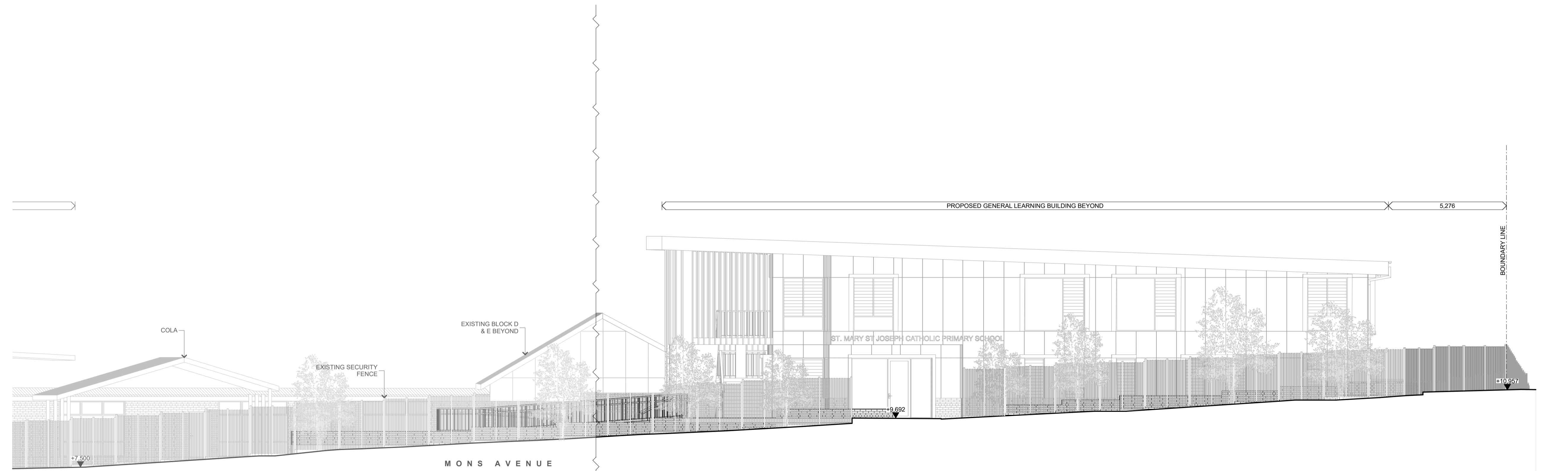
B MONS AVENUE STREET ELEVATION 1:100
